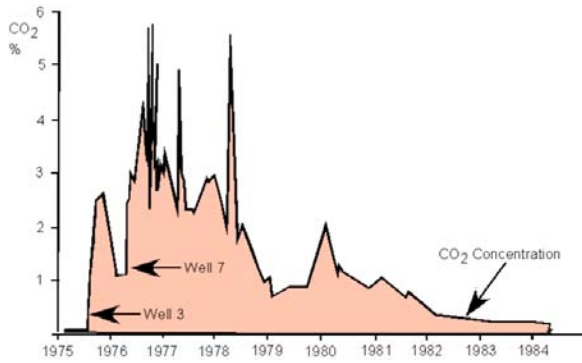
Figure 4: Changes in CO 2 concentrations in wells 3 and later the neighbouring well 7 during the Krafla fires 1975-1984
