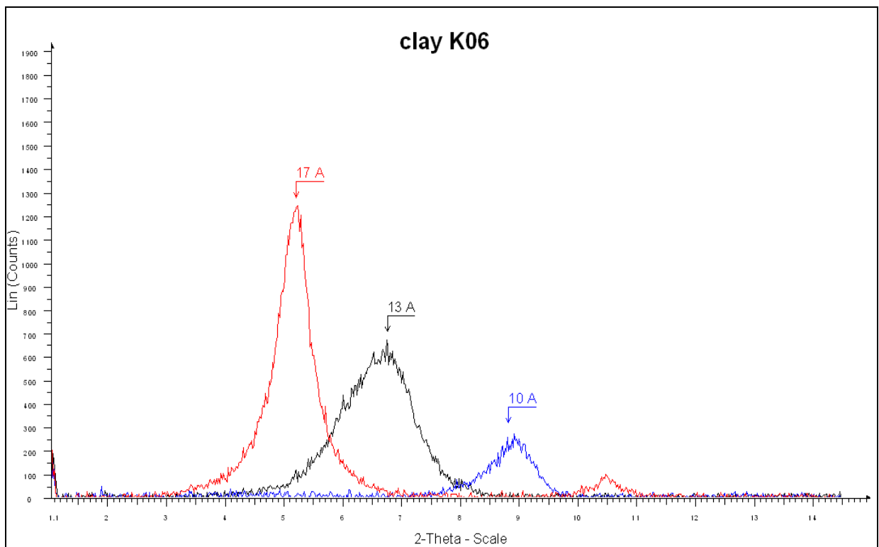
Figure 8: XRD pattern of a typical smectite in the altered core. The black line shows the untreated sample, the red line the glycolated sample and the blue line shows the pattern after heating the sample over 560°C.
